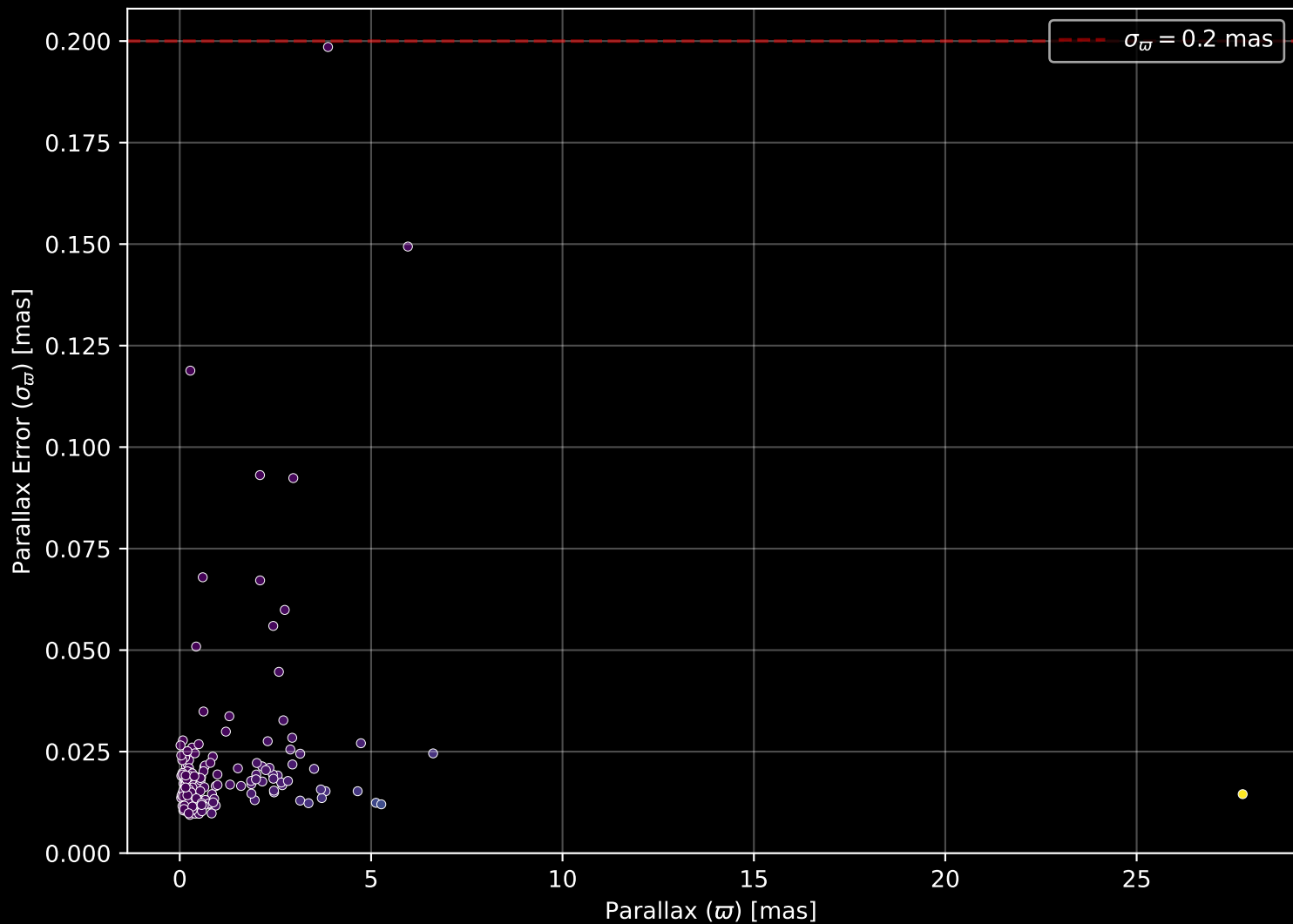
APOGEE DR17 Field: [064+12] Parallax Quality (n= 240)
