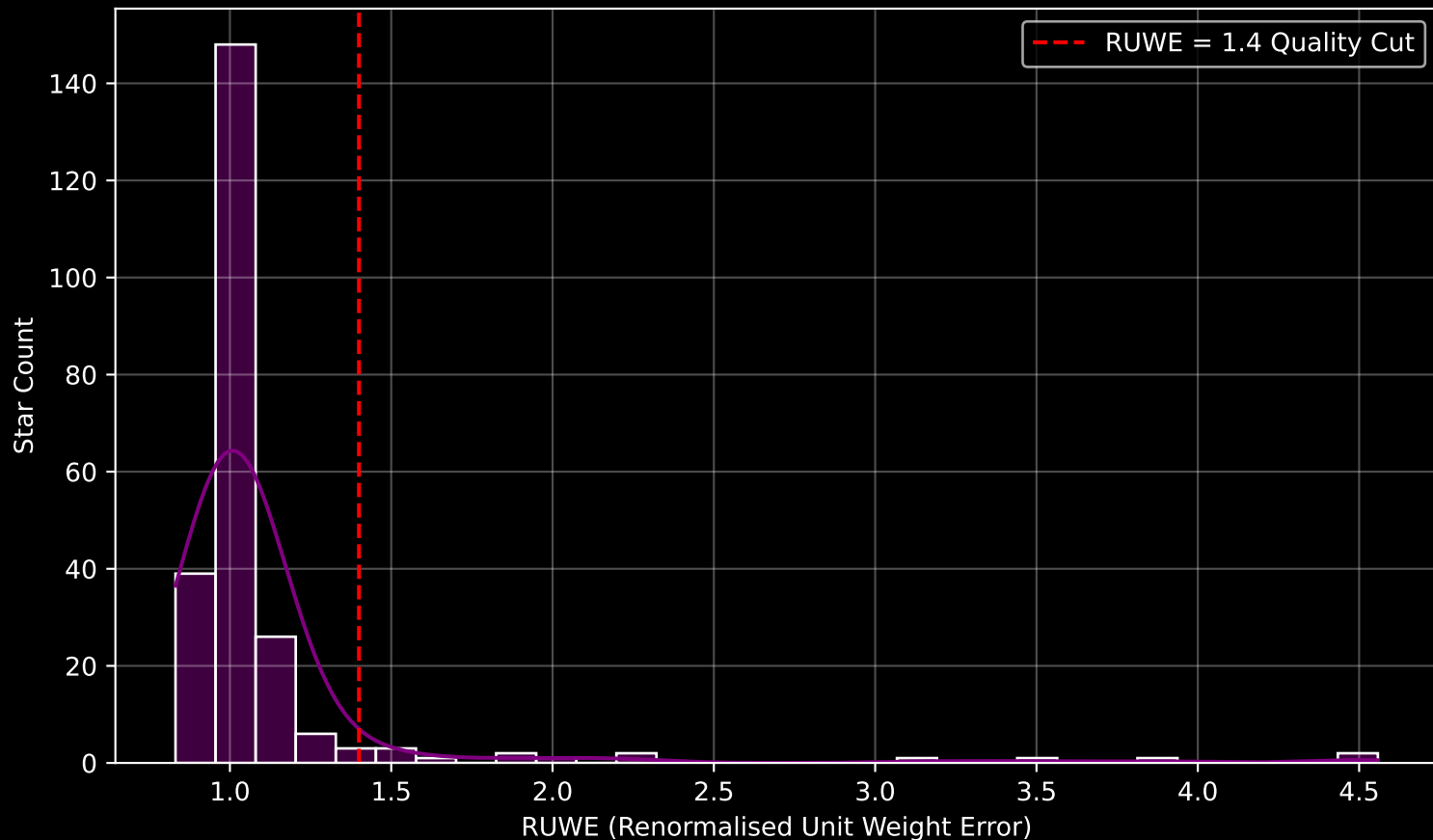
GAPOGEE DR17 Field [064+12] RUWE Distribution (n= 236)
