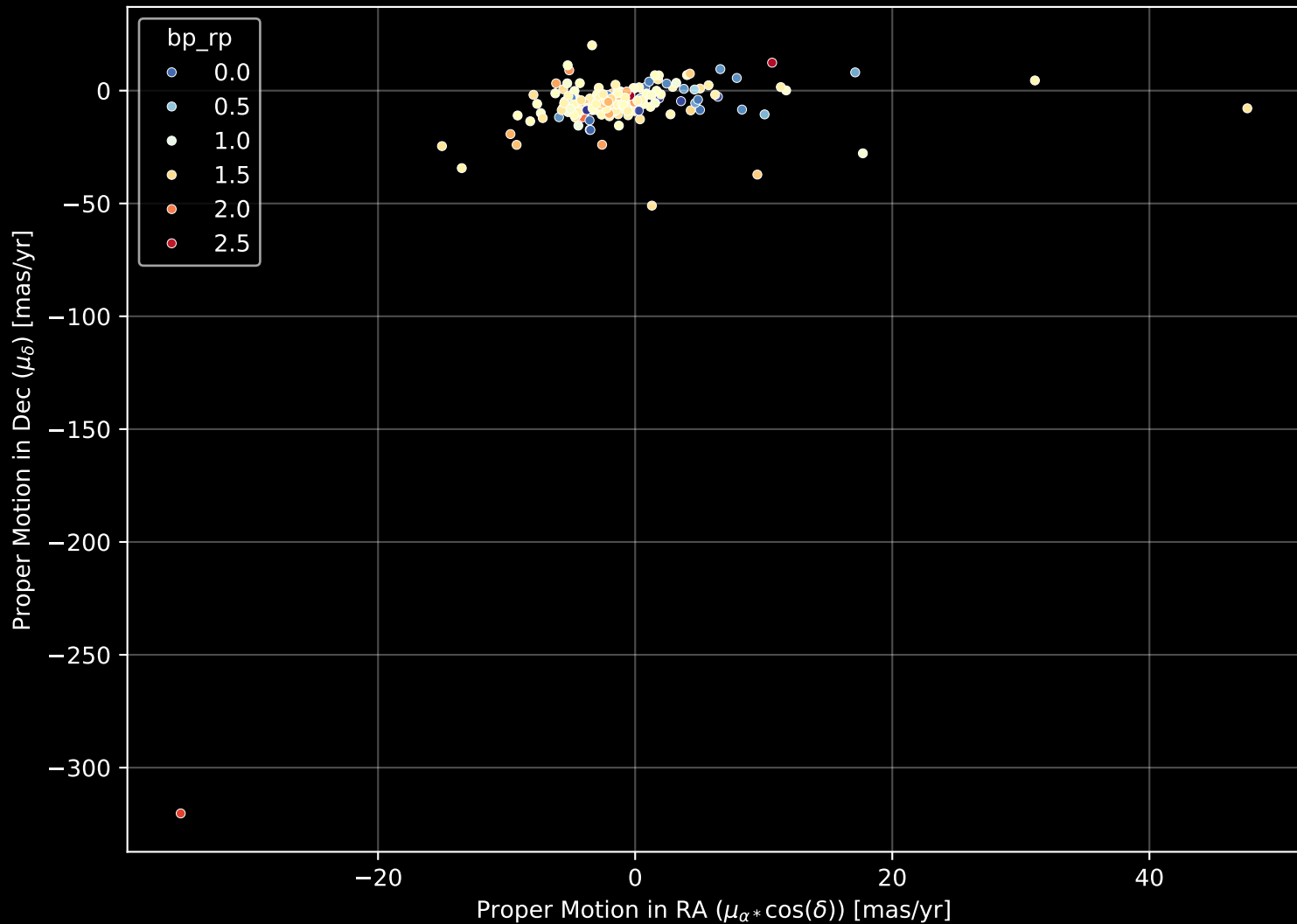
APOGEE DR17 Field: [064+12] Proper Motion Diagram (n= 240)
