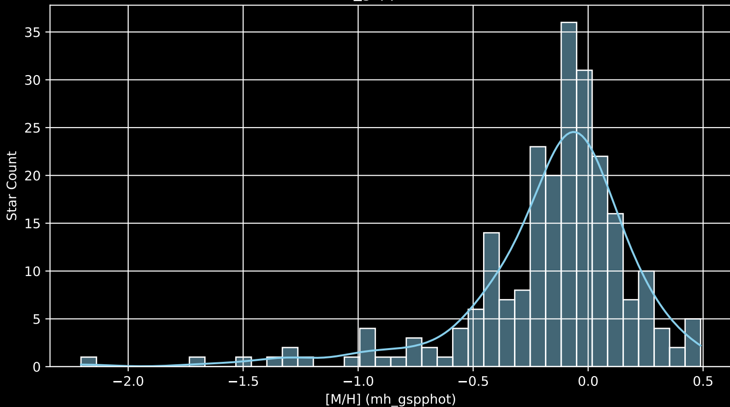
APOGEE DR17 Field: [064+12 [M/H] (mh_gspphot) (n= 235)
